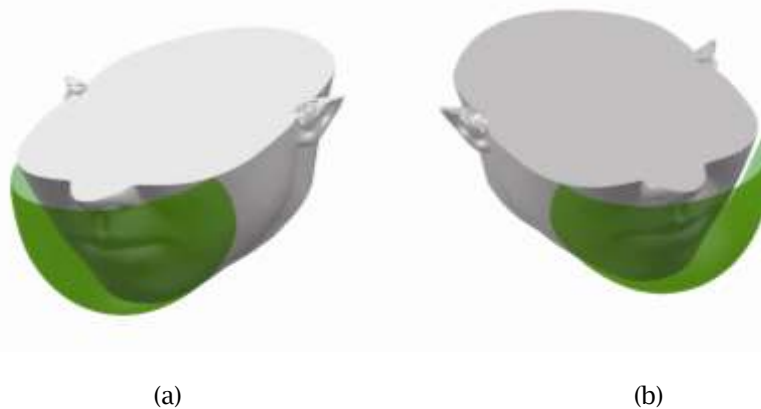
Fig. 13: Product fitting test in section view (a) A good fitting product (b) A poor fitting product
