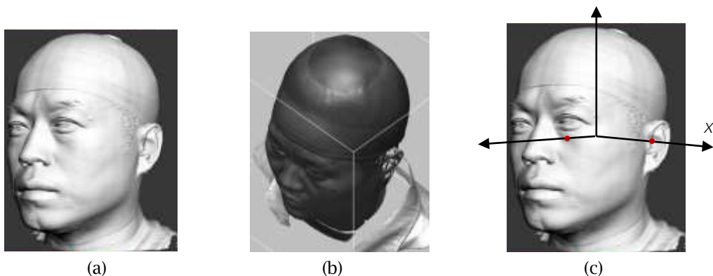
Fig. 1: Data processing
