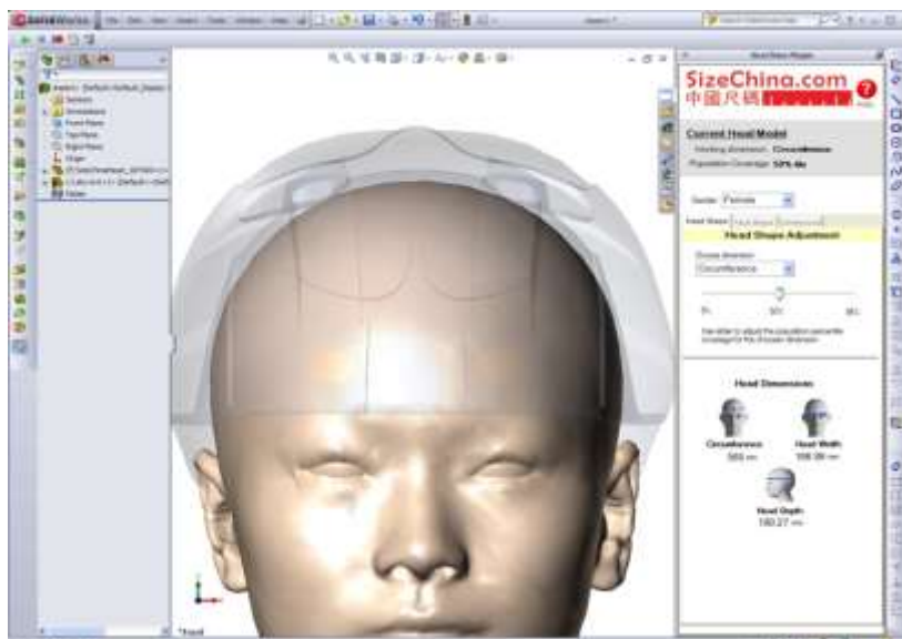
Fig. 10: Product fitting test between head template and product in a semi-transparent view
