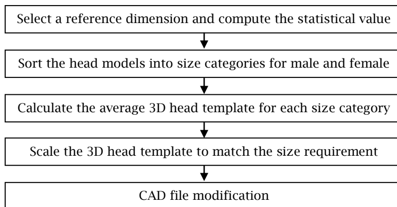
Fig. 2: Flow chart of head templates creation
