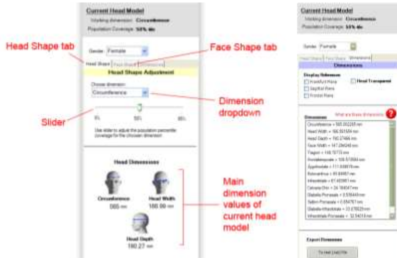
Fig. 9: Main user-interface of the design tool
