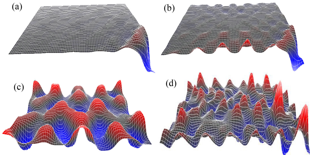
Fig. 15. Experimentally measured displacement distributions at selected frequencies as marked in Fig. 14 inside and outside the transmissibility attenuation band: (a) f=2831 Hz as marked by F_1 ; (b) f=3221 Hz as marked by F_2 ; (c) f=1562 Hz as marked by F_3 ; (d) f=4284 Hz as marked by F_4 . Excitation force is applied to the right bottom corner of the plate.
