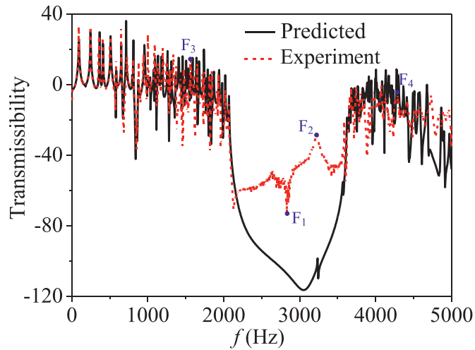
Fig. 14. Displacement transmissibility comparison between experimental (red dashed line) and numerical results (dark solid line). (For interpretation of the references to color in this figure legend, the reader is referred to the web version of this article.)
