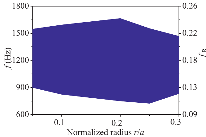
Fig. 11. Effect of normalized r/a on BGs.
