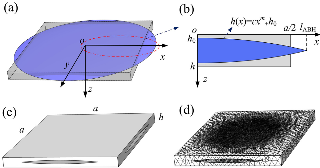
Fig. 2. (a) Unit cell of a periodic plate with a uniform plate element excavated inside by a symmetrical ABH circular cone as denoted by the blue solid; (b) local cross section of the unit cell as circled by the red dash line in Fig. 2(a), where the thickness of ABH profile follows h(x) = \epsilon x^m + h_0 ; (c) sketch of the unit cell; (d) FE mesh of the unit cell. (For interpretation of the references to color in this figure legend, the reader is referred to the web version of this article.)
