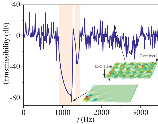
Fig. 7. Transmissibility of a finite plate with 6 \times 4 cells. Vibration displacement field is displayed for 1230 Hz and 2330 Hz, which are inside and outside attenuation band, respectively.
