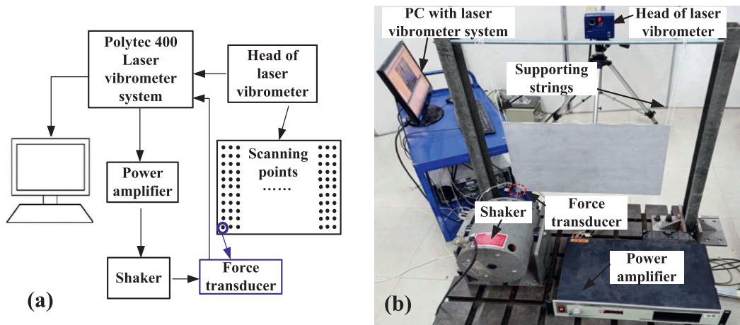
Fig. 13. Experimental system: (a) schematic diagram; (b) experimental setup.
