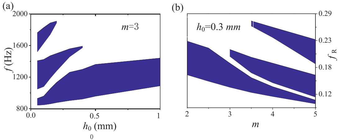
Fig. 8. Effect of (a) h_0 and (b) m on BGs as marked by blue areas. The upper and lower boundaries denote corresponding edge frequencies of the BGs. (For interpretation of the references to color in this figure legend, the reader is referred to the web version of this article.)
