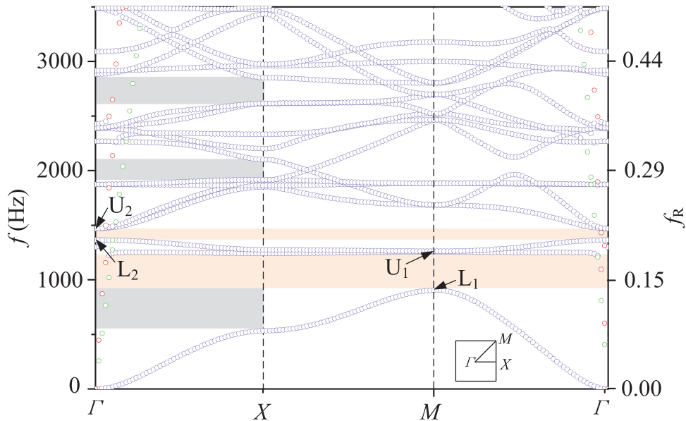
Fig. 3. Band structures with blue, red and green circles denoting flexural, S0 and SH0 waves, respectively. (For interpretation of the references to color in this figure legend, the reader is referred to the web version of this article.)
