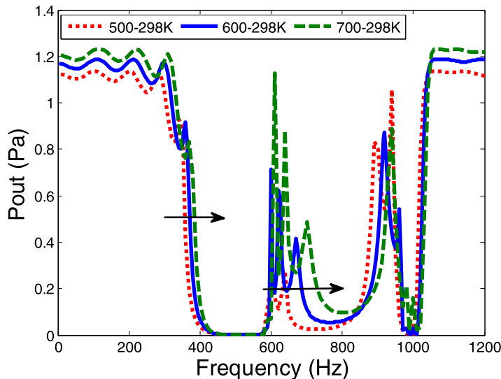
Fig. 5. Temperature gradient effect on the bandgap characteristics for three different temperature variations.
