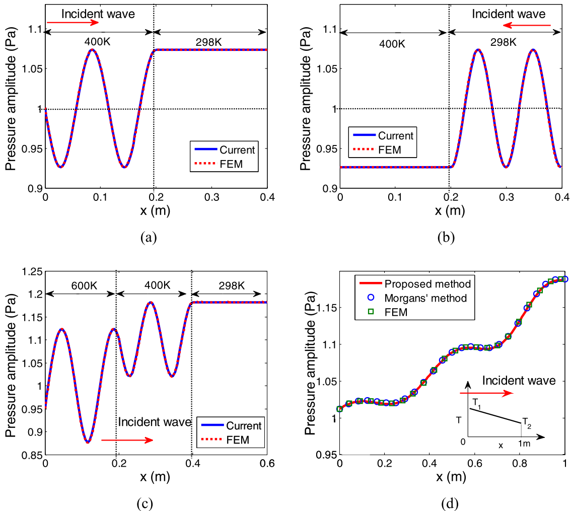
Fig. 2. Sound propagation predictions and comparisons with FE results. (a) Two temperature layers, incident wave from hot side. (b) Two temperature layers, incident wave from cold side. (c) Three temperature layers. (d) Linear mean temperature gradient with result from Morgans [28].
