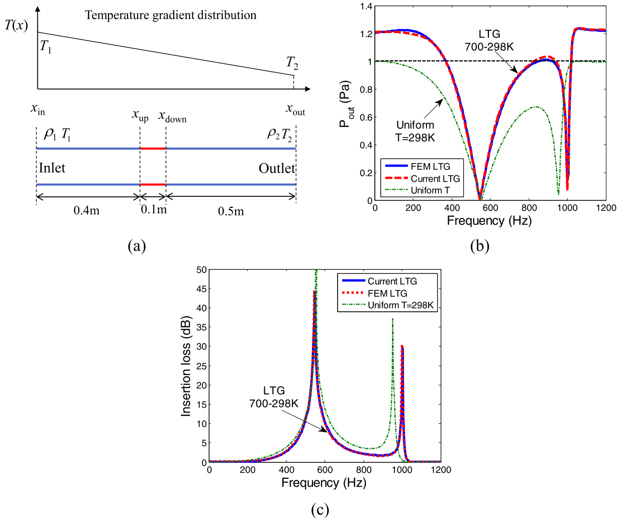
Fig. 3. Sound propagation for the duct-membrane system with a linear temperature gradient (LTG). (a) Schematic representation; (b) Transmission out sound pressure. (c) Insertion loss.
