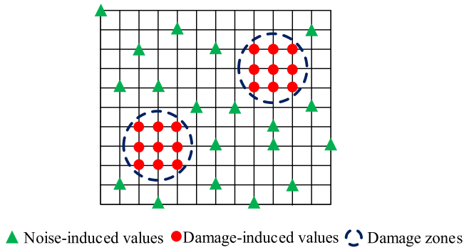
Figure 2. Illustration of outlier values of DI(x, y) .
