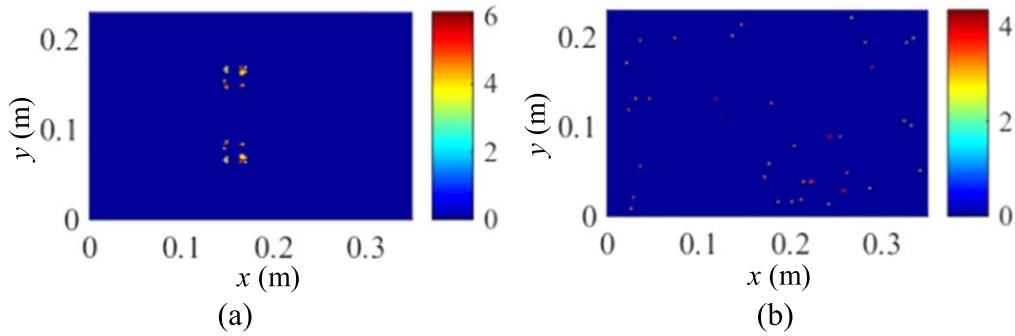
Figure 9. |DI(x, y)| by using the 10th mode for numerical case 2: (a) without noise effects and (b) with SNR = 60 dB.
