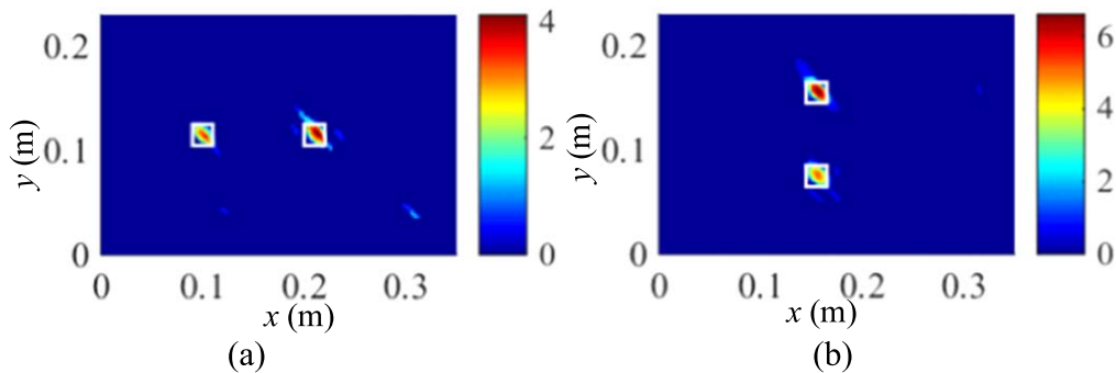
Figure 13. Integrated damage localization by using the 10th to 15th modes: (a) numerical case 1 and (b) numerical case 2.
