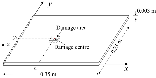
Figure 4. Configuration of a plate with damage.
