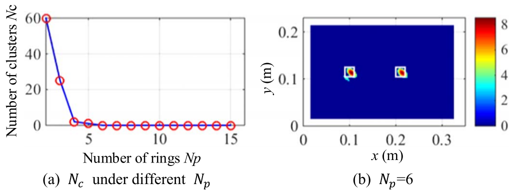
Figure 16. (a) Noise-induced clusters at different N_p and (b) damage localization results when using N_p = 6 for experimental case 1.
