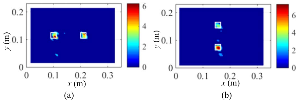
Figure 18. Integrated damage localization results: (a) experimental case 1 and (b) experimental case 2.
