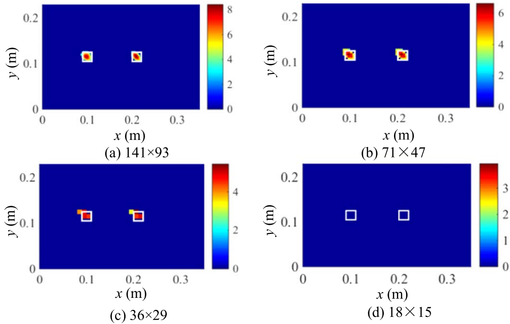
Figure 11. Damage localization results on numerical case 1 based on the 10th mode shape using different measurement points.
