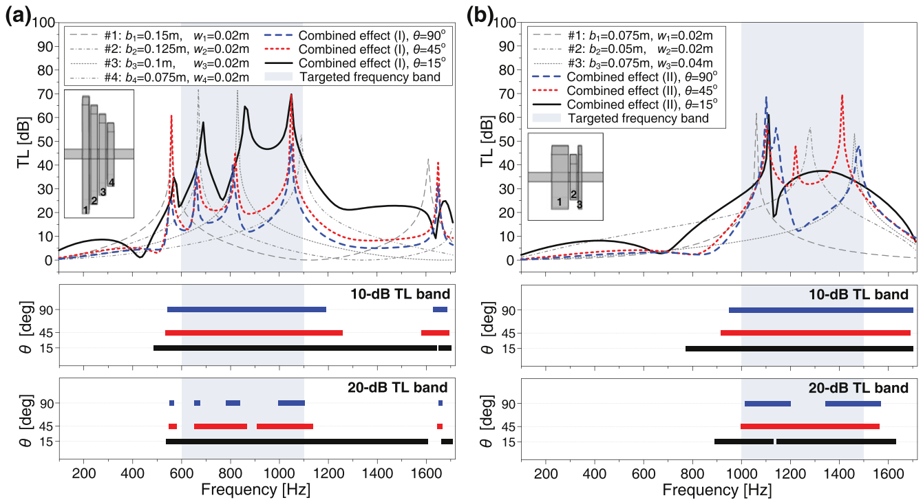
Figure 10. Two examples showing the programmability and modularization concepts based on the combined effect of cascading multiple optimized silencer layers. The targeted frequency band (shaded) for (a) and (b) are [600, 1100] Hz and [1000, 1500] Hz, respectively. From the top to the bottom shows the TL curves, the 10 dB TL band, and the 20 dB TL band, respectively. For illustration purpose, TL curves of the constituent layers at the \theta = 15^\circ configuration are provided; TL curves of the multi-layer silencer at the \theta = 90^\circ , \theta = 45^\circ , and \theta = 15^\circ configurations are given.
