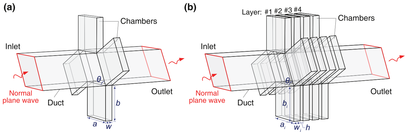
Figure 2. Conceptual designs of (a) a single-layer origami silencer and (b) 4-layer origami silencer. Chambers within each layer share the same dimensions.
