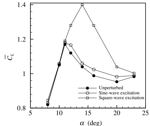
Fig. 5 Mean lift coefficient \bar{C}_L vs angle of attack \alpha with and without perturbation.
