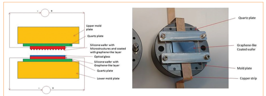
把鍍上類石墨烯的硅片加熱 Heating of graphene-like coated wafer
