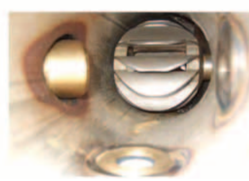
安裝在水管內的噴嘴和葉輪，入水口（上圖）和出水口（下圖） The nozzle and impeller installed inside the pipe, viewed from the water entry (top) and water exit (bottom) side respectively
