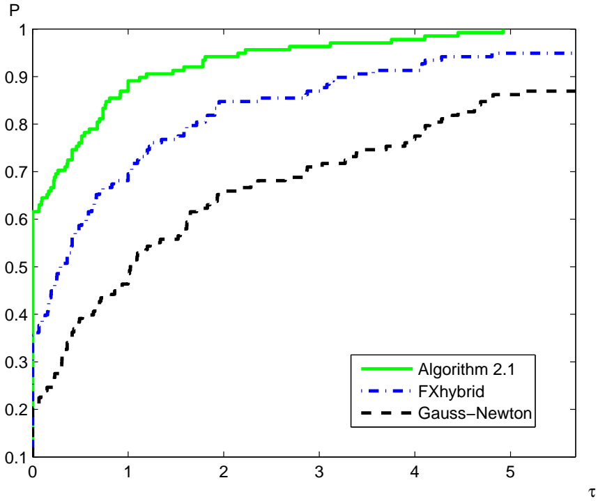
Figure 1: Performance profiles with respect to the number of iterations.
