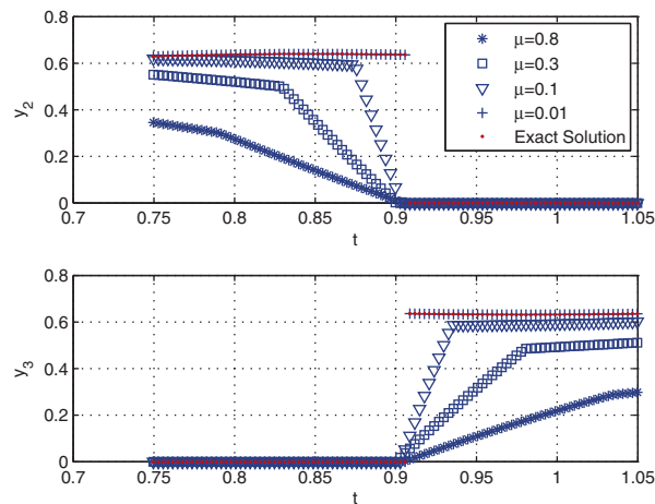
FIG. 3. Numerical results for y_2(t) and y_3(t) .
