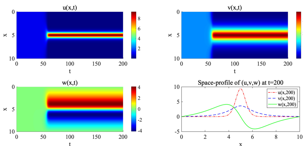
Figure 1: Spatio-temporal patterns generated by the system (1.2)-(1.3) in the interval \Omega = [0, 10] with \chi = 5, \varepsilon = 1 , where the initial value (u_0, v_0, w_0) is given by (4.9) with m = 1 .
