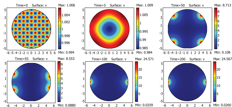
Figure 3: Time evolution patterns of v(x,t) generated by the system (1.6) in a disk with radius 5 centered at the origin, where \chi=5, \lambda=1 and \varepsilon=1 . The initial value (u_0, v_0, w_0) is chosen as u_0 = v_0 = 1 + 0.01 \cdot \cos(\pi x) \cdot \cos(\pi y), w_0 = 0 .
