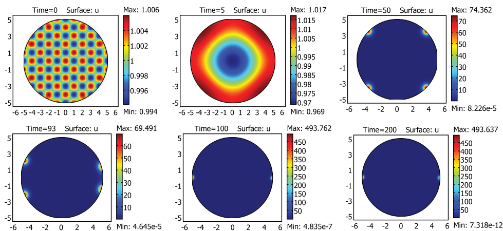
Figure 2: Time evolution patterns of u(x, t) generated by the system (1.6) in a disk with radius 5 centered at the origin, where \chi = 5 , \lambda = 1 and \varepsilon = 1 . The initial value (u_0, v_0, w_0) is chosen as u_0 = v_0 = 1 + 0.01 \cdot \cos(\pi x) \cdot \cos(\pi y) , w_0 = 0 .
