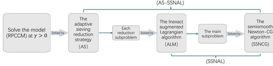
Figure 2: The overall structure of AS-SSNAL for solving the model (RPCCM).
