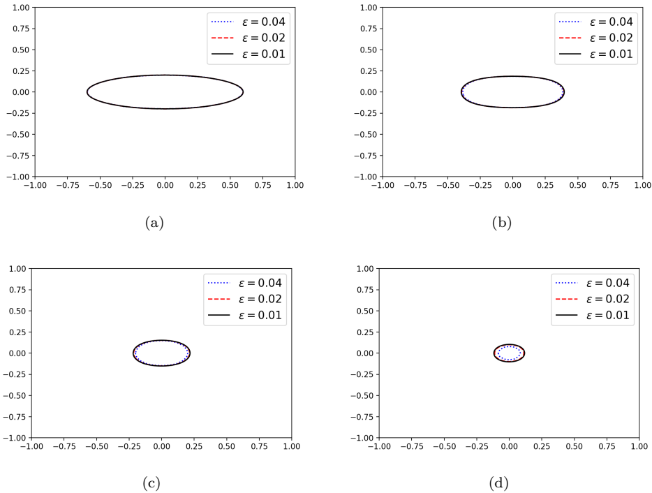
Fig. 2. Snapshots of the zero-level set of u_h^n at time t = 0, 0.02, 0.04, 0.05 , \tau = 0.5\varepsilon^2 and \varepsilon = 0.04, 0.02, 0.01 .
