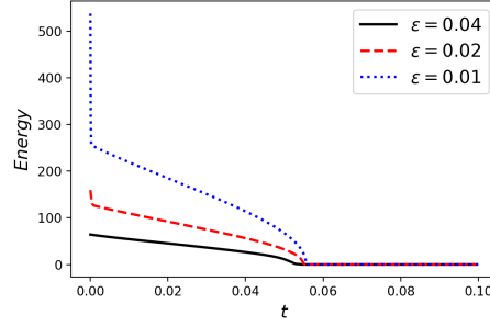
Fig. 3. Energy evolution of numerical solutions, with \tau = \varepsilon^2 and h = \varepsilon/\sqrt{2} .
