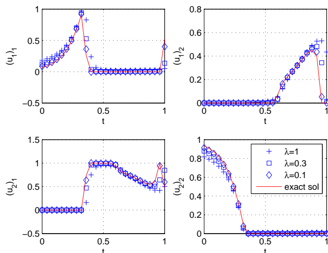
Fig. 3 Numerical results for u(t) with \mu = \lambda^2
