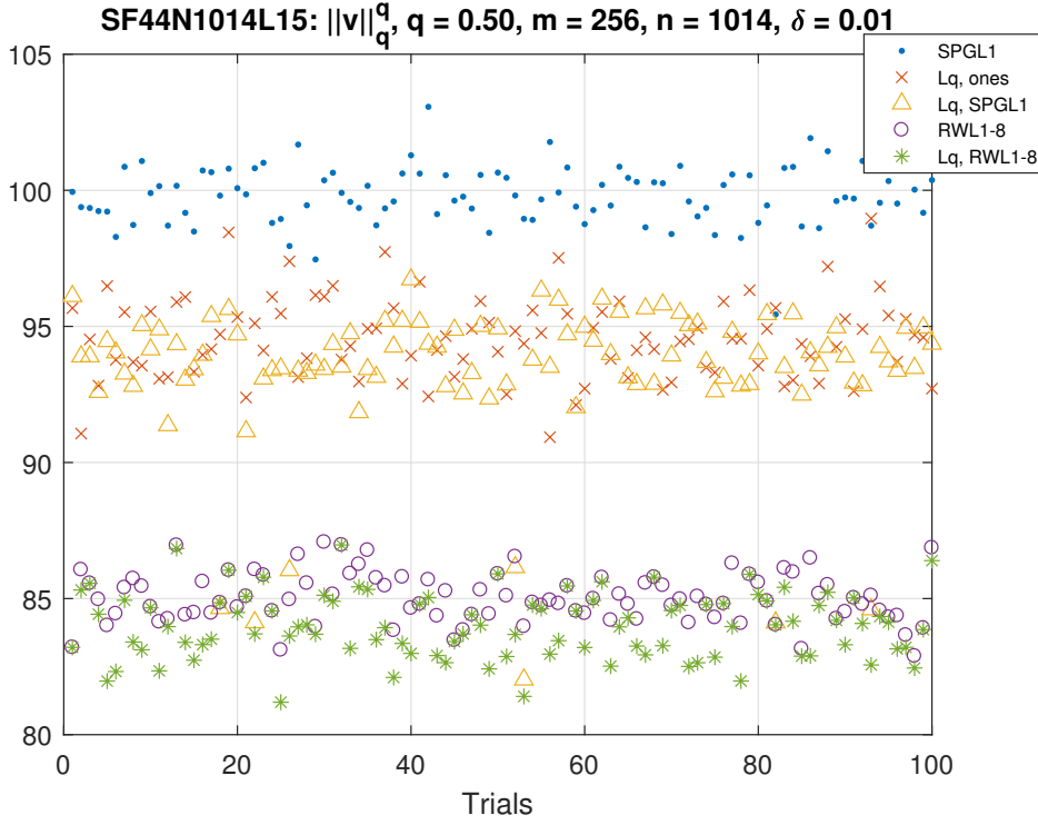
FIG. 8. Values of \|v\|_q^q at the calculated solutions using SF nodes: m = 256 , n = 1014 , q = 0.5 , |J^*| = 120 , for 100 trials with \delta = 0.01 . The values of \|v\|_q^q at the randomly generated sparse solution v^* is \|v^*\|_q^q = 84.639 .
