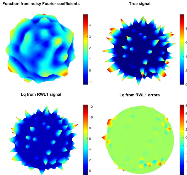
FIG. 10. MD nodes: function from noisy Fourier coefficients, true signal, signal minimizing \|v\|_q^q from solution of Algorithm 4.1 with k^* = 8 , and error
