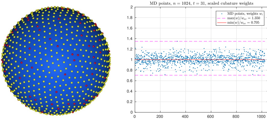
FIG. 4. MD points and cubature weights
