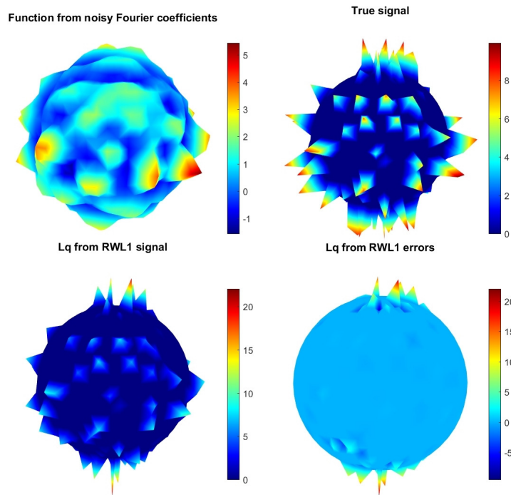
FIG. 11. GL nodes: function from noisy Fourier coefficients, true signal, signal minimizing \|v\|_q^q from solution of Algorithm 4.1 with k^* = 8 , and error
