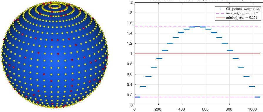
FIG. 5. GL points and cubature weights
