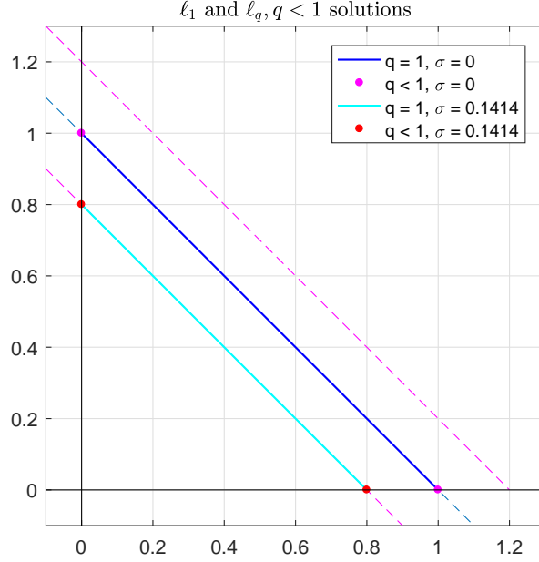
FIG. 2. Example 1.1 with multiple solutions for q = 1 and q \in (0, 1) : S_1 = \{(v_1, 1 - \sqrt{2}\sigma - v_1)^T, v_1 \in [0, 1 - \sqrt{2}\sigma]\} containing a segment between (0, 1 - \sqrt{2}\sigma)^T and (1 - \sqrt{2}\sigma, 0)^T , and S_q = \{(0, 1 - \sqrt{2}\sigma)^T, (1 - \sqrt{2}\sigma, 0)^T\} containing only two points.
