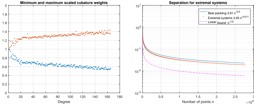
FIG. 7. Scaled cubature weights and separation for maximum determinant systems
