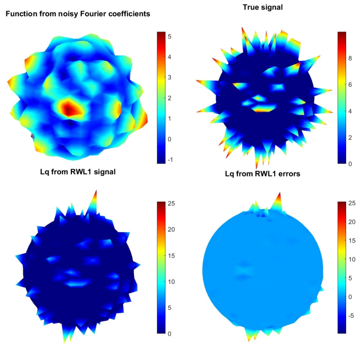
FIG. 12. TP nodes: function from noisy Fourier coefficients, true signal, signal minimizing \|v\|_q^q from solution of Algorithm 4.1 with k^* = 8 , and error
